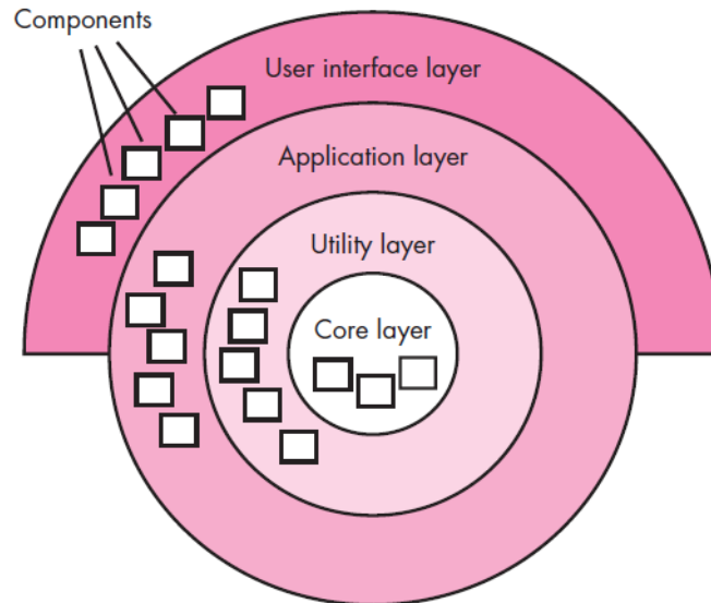
Fig 9.4: Layered architecture
