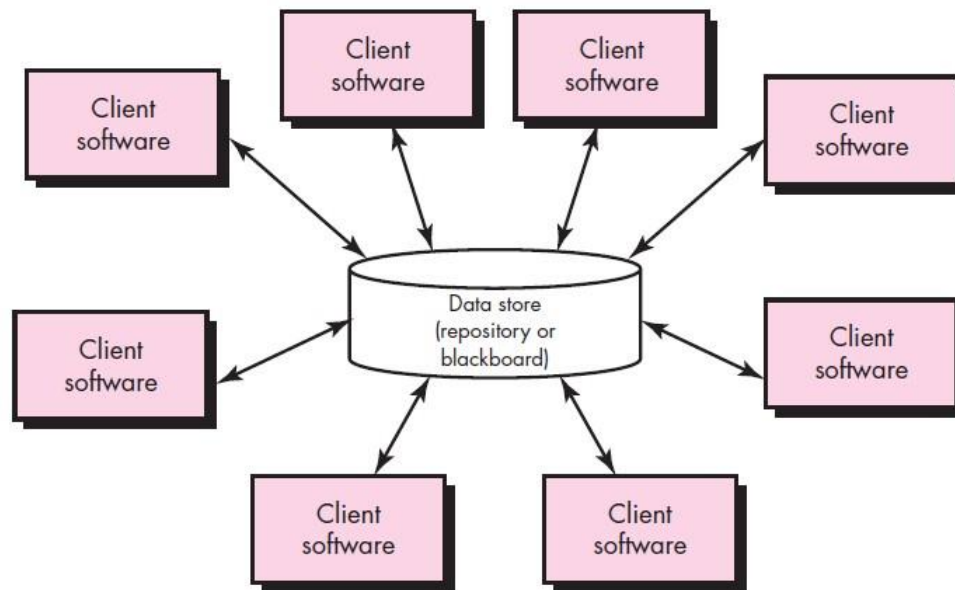
Fig 9.1: Data-centered architecture
