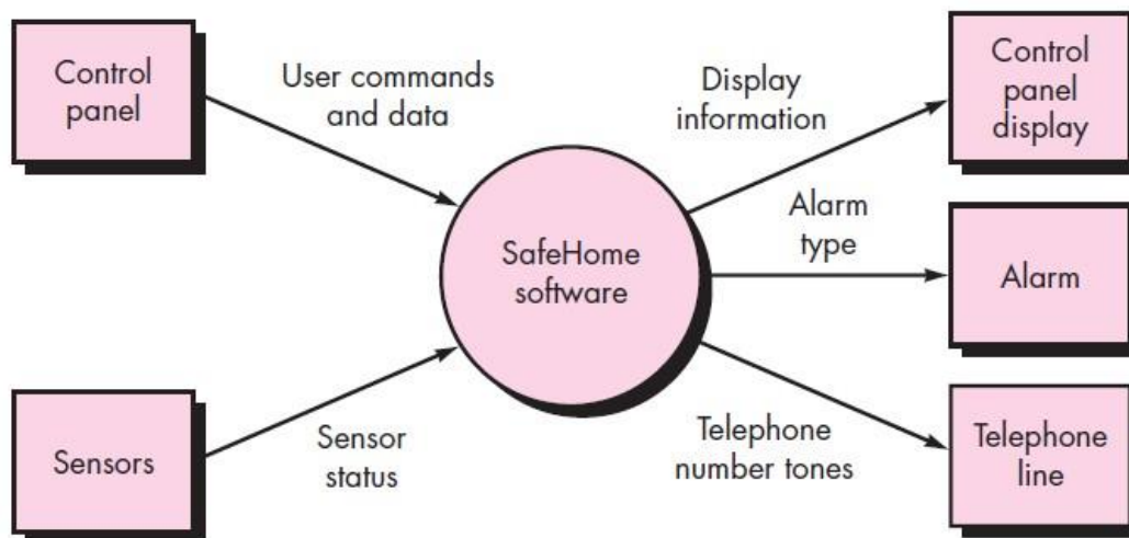
Fig 9.10 Context-level DFD for safeHome security function
